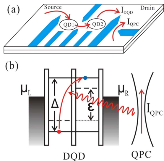
FIG. 1. (Color online) (a) Schematic of a DQD connected to two electrodes via tunneling barriers. A QPC used for measuring the electron states yields backaction on the DQD. (b) QPC-driven interdot electronic transition between two DQD eigenstates with an energy difference \Delta . The energy detuning \varepsilon between the two single-dot levels (dashed lines) can be varied by tuning the gate voltages.
